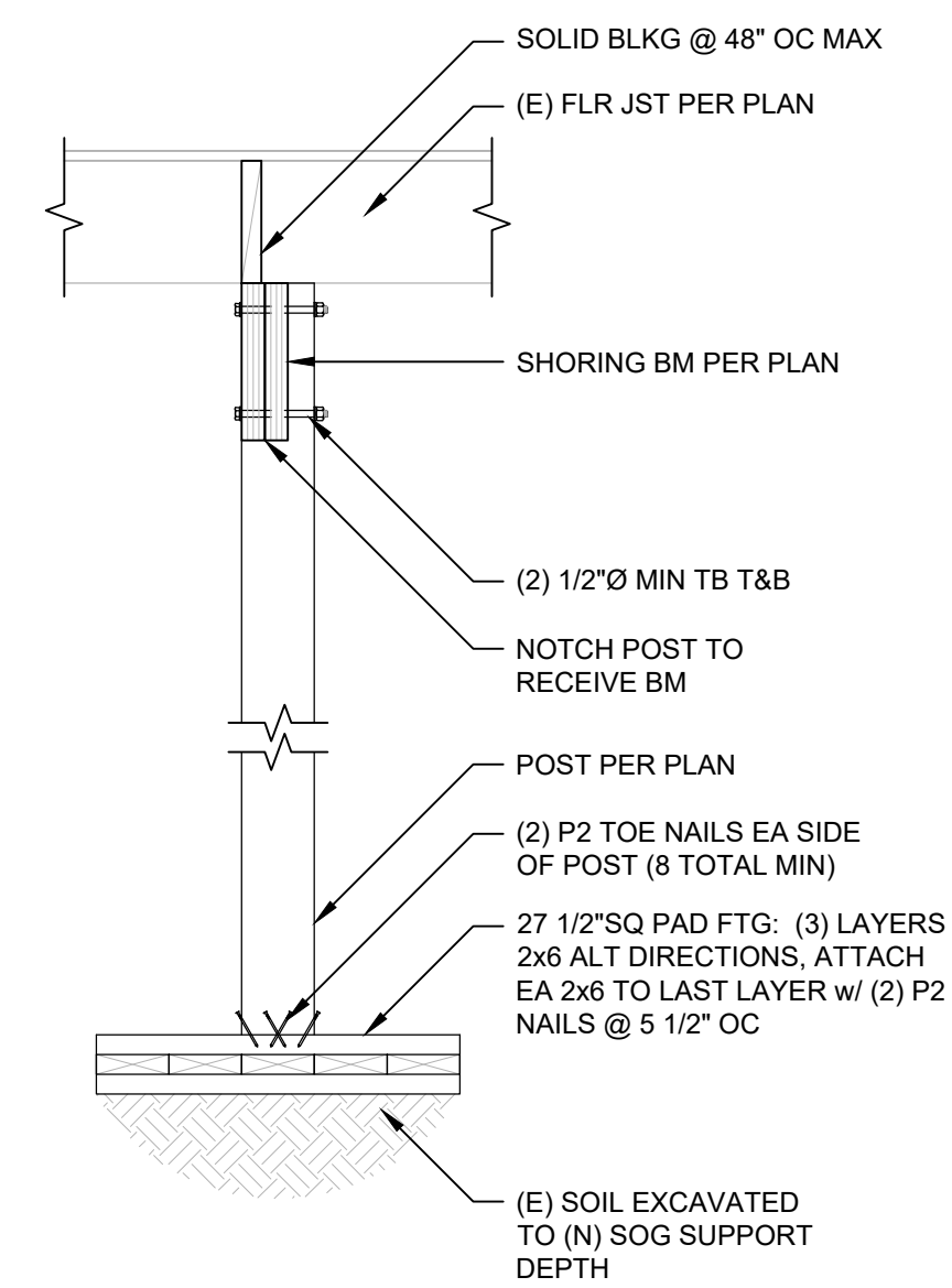
1 TYP SHORE POST & PAD SCALE: 3/4" = 1'-0" RE: SH-1
